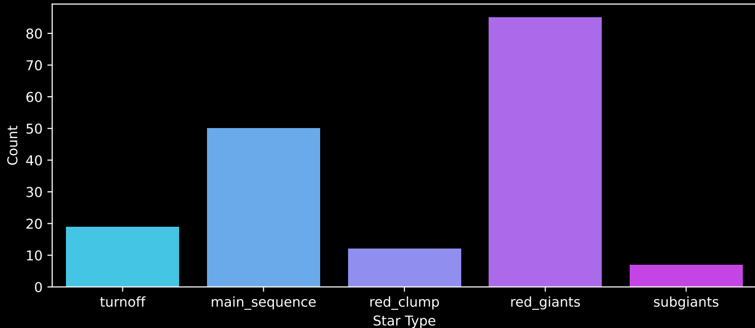
APOGEE DR17 Field: [280+49] Count plot of Star Type
