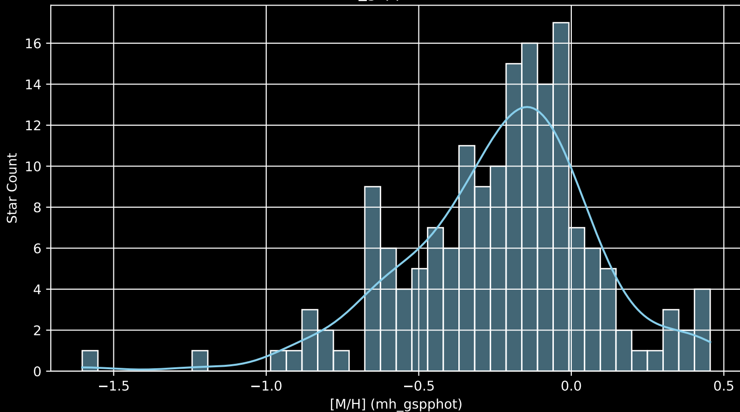
APOGEE DR17 Field: [280+49 [M/H] (mh_gspphot) (n= 170)
