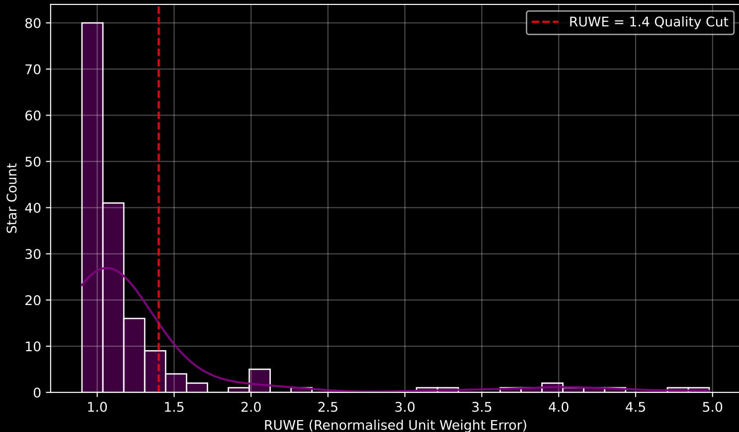
GAPOGEE DR17 Field [280+49] RUWE Distribution (n= 170)
