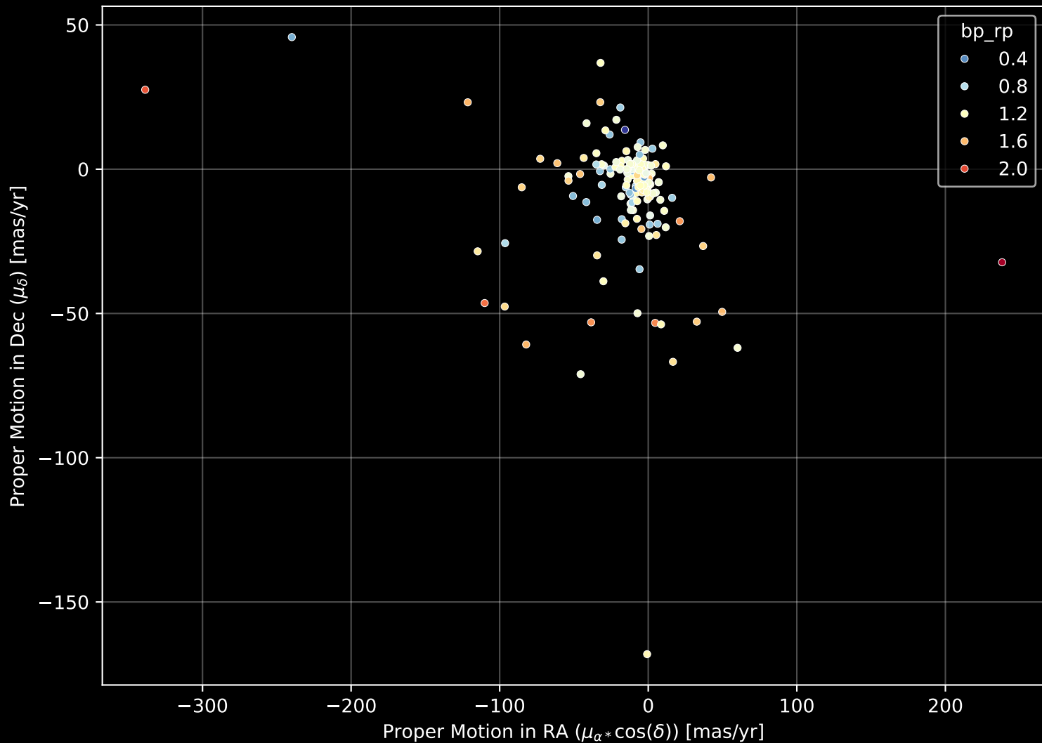
APOGEE DR17 Field: [280+49] Proper Motion Diagram (n= 173)
