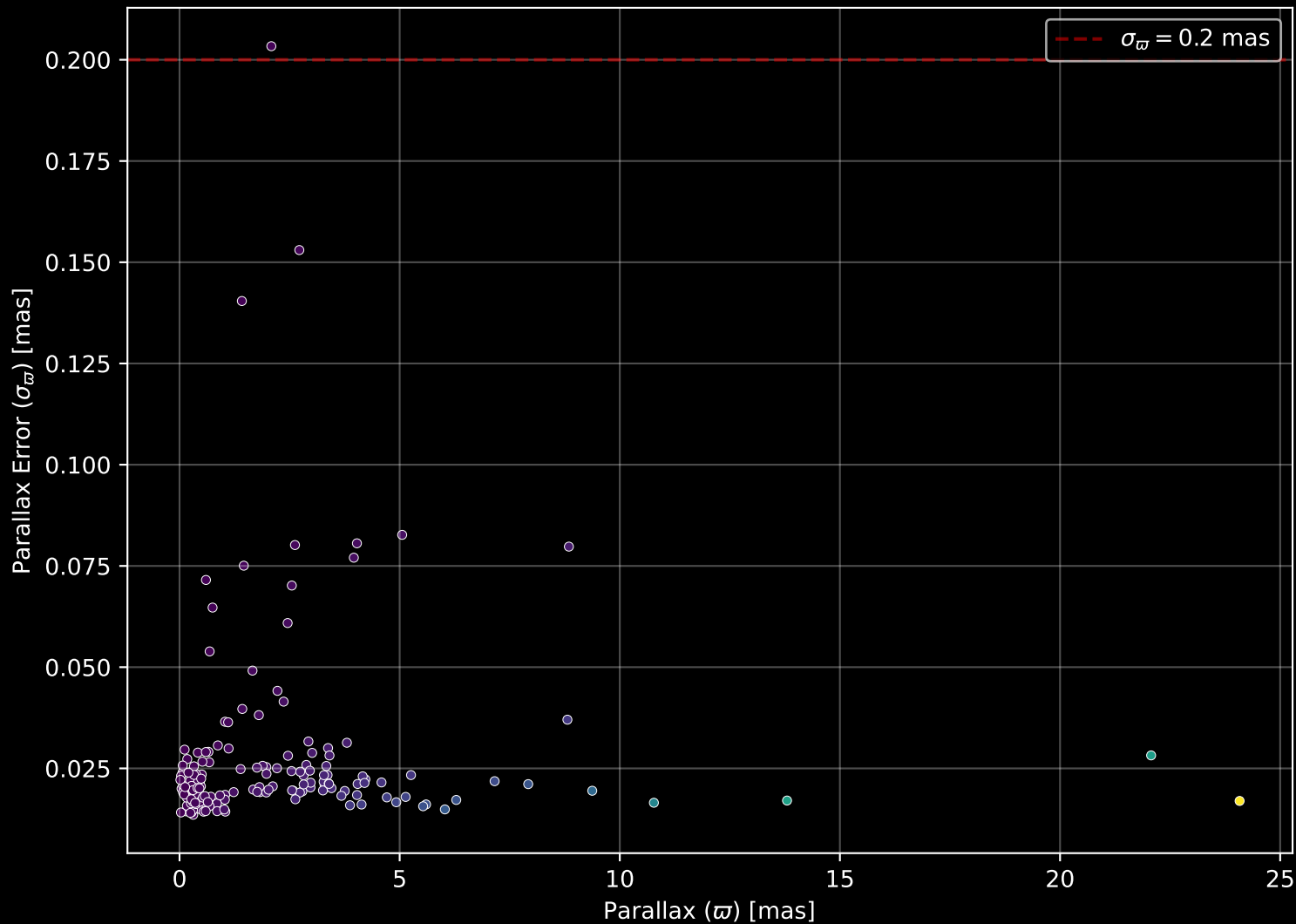
APOGEE DR17 Field: [280+49] Parallax Quality (n= 173)
